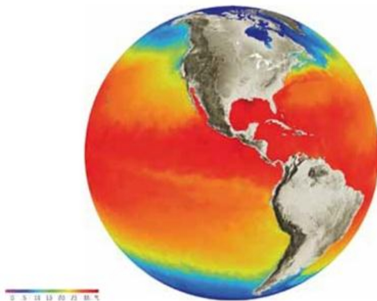
Figure 4-2: Global SST map derived from a combination of data derived from the (A)ATSR reference SST satellite instruments, in situ measurements and other satellite SST datasets. SENTINEL-3 will maintain and extend the high-quality SST measurements of the (A)ATSR series required by Copernicus and other climate services. (Credit: Met Office, UK)
