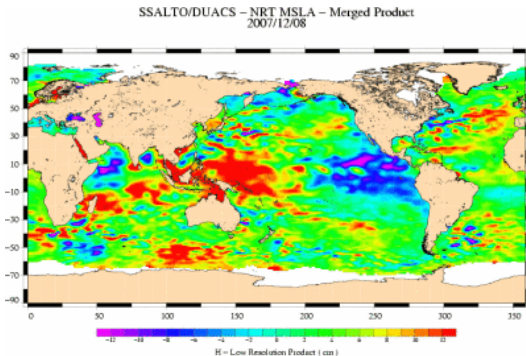
Figure 2-4: The variation of MSL anomalies on a global scale. Positive anomalies indicate more heat content (warmer waters, a deeper thermocline) whereas negative anomalies indicate less heat content (cooler waters, a shallower thermocline). Generally, sea level is higher than average in the northern hemisphere in July and August when waters are warmed by more direct solar radiation and is lower than average in February and March when the incoming solar flux reduces. These sea level anomalies maps derive from a combination of data coming from altimeters on-board JASON-1 and ENVISAT. Feb 2007-Dec 2008 (Credit: CNES/CLS)
