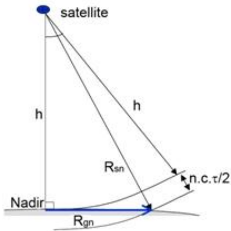
Figure 2-27: LRM Footprint (Credit: TAS-F)
