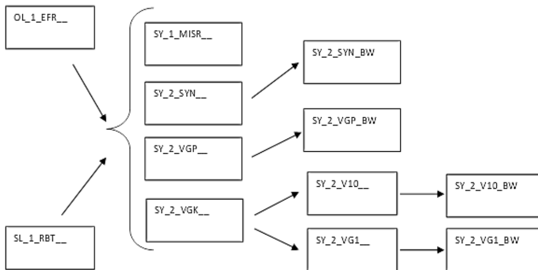
Figure 5-4: Synergy Product Tree
