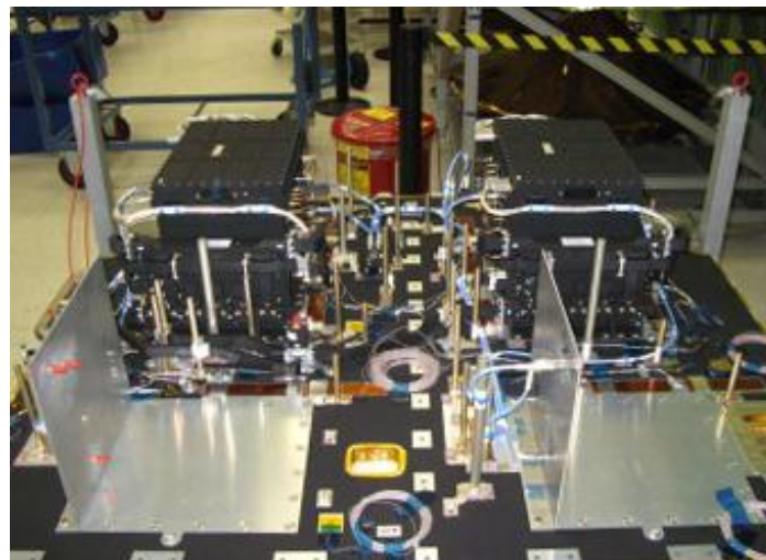
Figure 1-10: SRAL Instrument (Credit: ESA)
