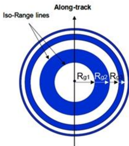
Figure 2-29: SAR Range Gates (Credit: TAS-F)
