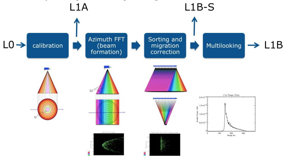
Figure 2-24: Level-1 High Resolution (SAR) Processing steps (Credit: ESA)
