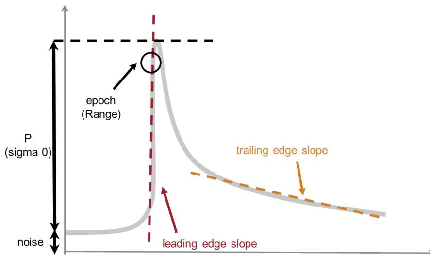
Figure 2-3: Physical Characteristics of the Altimetry Waveforms (Credit: isardSAT)
