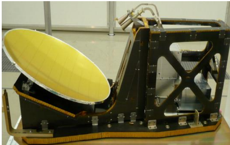
Figure 1-11: MWR Instrument (Credit: ESA)
