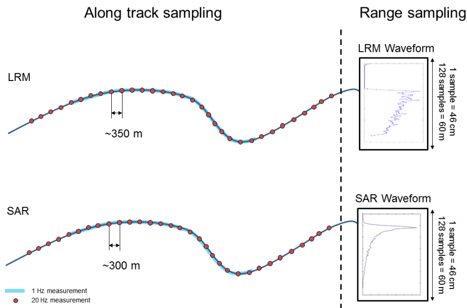
Figure 2-26: LRM and SAR Along Track Sampling at 1 Hz and 20 Hz Measurement Rate (left) and Range Sampling (right) (Credit: Thales Alenia Spazio)
