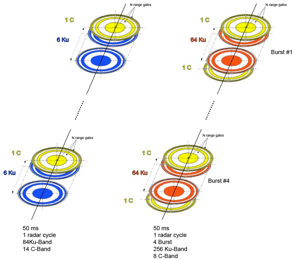
Figure 2-25: LRM radar cycle transmitting pattern (left) and SAR radar cycle transmitting pattern (right) LRM radar cycles contain 96 pulses (84 Ku-band and 14 C-band) structured in transmitting sequences of 1 C - 6 Ku pulses. SAR radar cycles contain four bursts, each of these bursts structured in transmitting sequences of 1 C - 64 Ku - 1 C pulses. (Credit: Thales Alenia Spazio).
