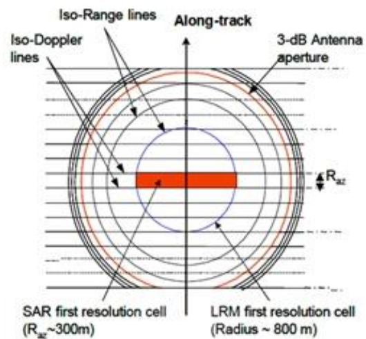
Figure 2-30: SAR Resolution Cell (Credit: TAS-F)
