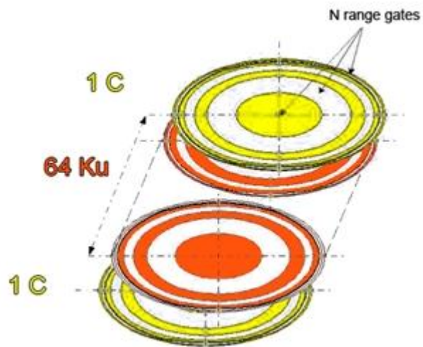
Figure 2-28: LRM Resolution Cell (Credit: TAS-F)
