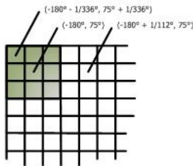
Figure 5-6: SPOT VGT 1 km Plate-Carrée Grid Cell
