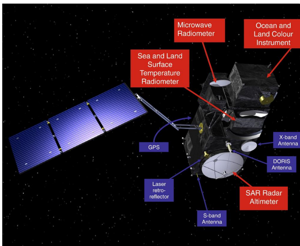
Figure 1-7: Sentinel-3 Payloads (credit:ESA)
