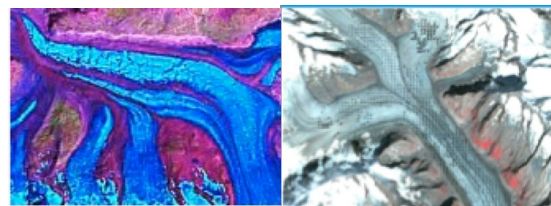
Glaciers & Ice
