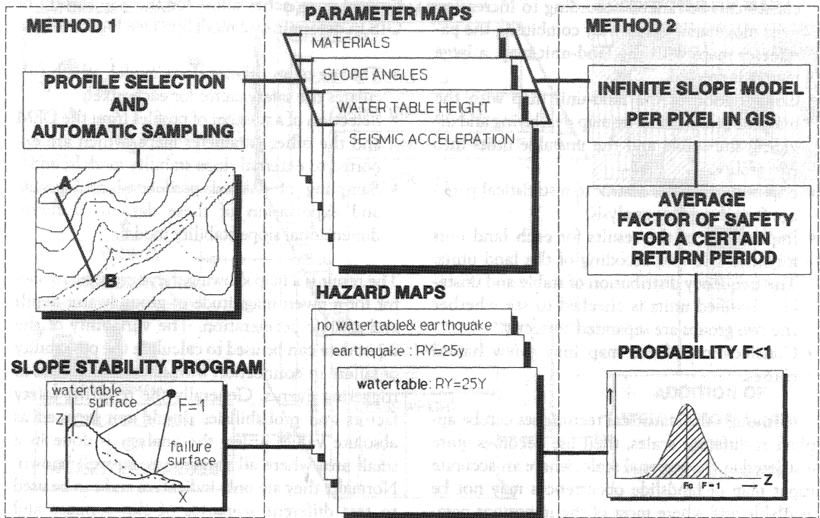
FIGURE 8-19 Use of GIS in deterministic analysis.
