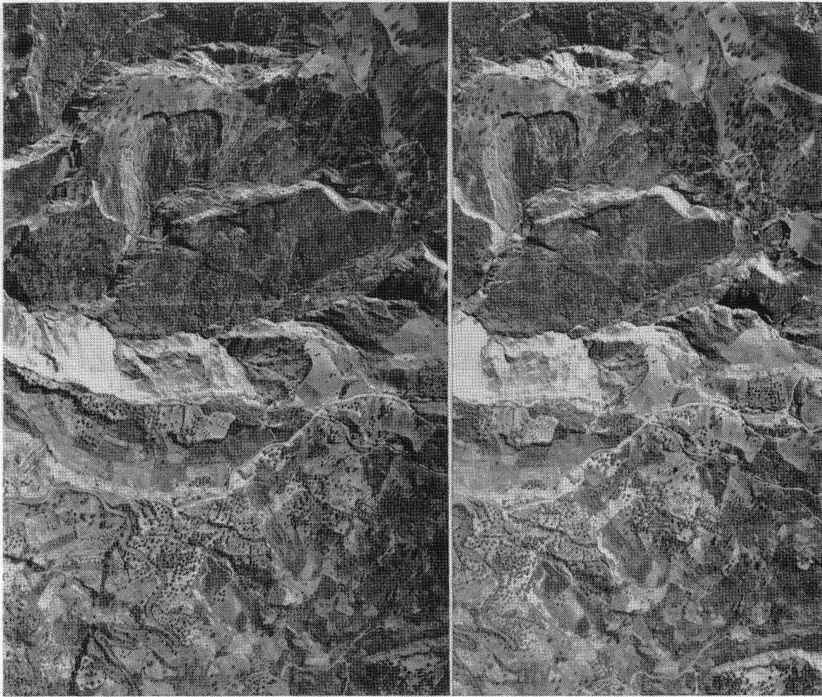
FIGURE 8-4 Translational slides controlled by dip slopes in sequence of very friable sandstones alternating with siltstones and mudstones. Joint-controlled back scarp, linear patterns, and micromorphology of area where the sandstones have slid away ( lower part ) are diagnostic for landslides. Somewhat comparable morphology and change in land use ( upper part ) are indicative of landslides that have rapidly transformed into earth flow because of higher clay content (original photograph scale 1:17,000, Basilicata, Italy).
